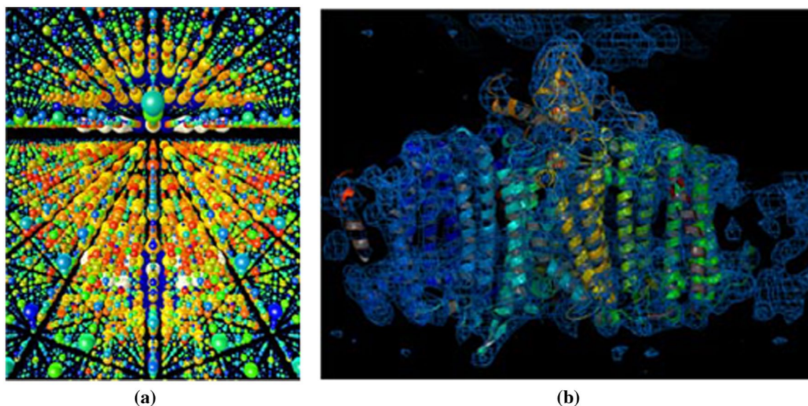
Figure 37. (a) Three-dimensional rendering of the X-ray diffraction pattern for the Photosystem I protein, reconstructed from more than 15,000 single nanocrystal snapshots taken at the LCLS. Credit: Thomas White, DESY. (b) A reconstructed image of the Photosystem I complex. Credit: Raimund Fromme, Arizona State University. Reprinted with permission from [97]. Copyright: American Physical Society.
