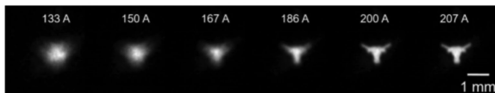
Figure 24. Imaging of metastable neon atoms using a pulsed hexapole magnetic lens. The complex pattern formed is easily recognized in the last frame (Image courtesy of Erik Ancaux, Raizen Laboratory).
