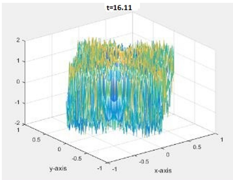
Figure 31. A snapshot of chaotic vibrations on a 2D domain excerpted from [151]). For a video animation, please see video animation of chaotic vibrations on a 2D domain. The main objective of the work is to show the complexity of spatiotemporal chaos and to perform mathematical analyses of chaos in multidimensional settings; at present, it has no specific applications.
