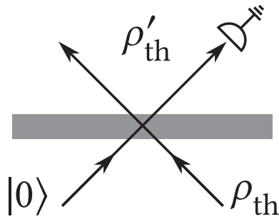
Figure 19. Model of a black hole as a beam splitter to obtain the Bekenstein entropy formula. Here, the two input modes are in the vacuum state |0\rangle and a thermal state \rho_{\text{th}} of a given average number of photons, and the output modes are either absorbed or in a thermal state \rho'_{\text{th}} corresponding to a number of photons that is smaller than of \rho_{\text{th}} . Credit: Harald Losert.
