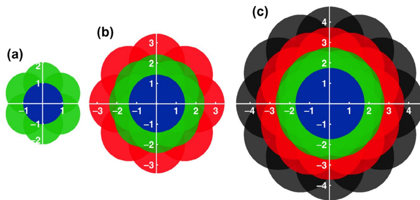
Figure 27. (a)–(c) Comparison of the observable regions in reciprocal space provided by ordinary structured illumination microscopy [SIM], structured illumination quantum correlation microscopy [SIQCM] of order two and three (left to right). The axes are normalized by the modulus of the highest spatial frequency k_{\text{max}} \equiv 1 transmitted through the imaging system. The green discs stem from the densities \tilde{n}(k \pm k_0) , while the red and black discs originate from the higher harmonics arising in the SIQCM different order signals. Note that the size of the individual discs is enlarged from (a) to (c) (after [72]) because of correlations of different order.
