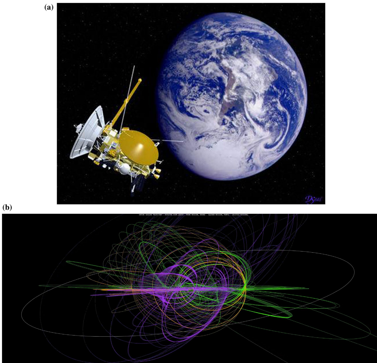
Figure 30. Non-linear trajectories in the Cassini-Huygen's space mission: (a) The Earth-Moon fly-by of the Cassini spacecraft gave a 5.5 km/second speed boost, so although the craft was once again only 1,100 km from Earth after almost 2 years of travel, its speed was considerably greater. (b) Mission planners referred to the trajectories of Cassini as “the ball of yarn”. All orbits between 1 July 2004 and 15 September 2017 are shown in this image. Cassini's mission terminated in September 2017. Credit: NASA.
