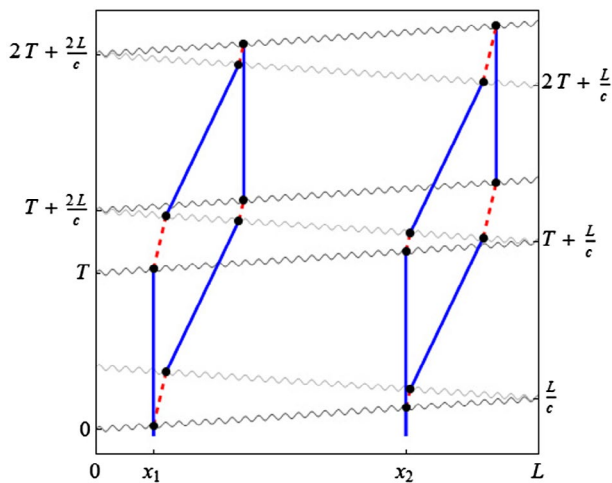
Figure 16. Laser interferometers. Credit: Surjeet Rajendran.
