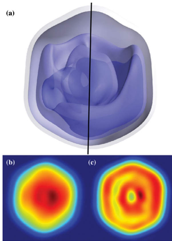
Figure 38. Reconstructed electron density from [78], reproduced with permission. (a) The electron density of the mimivirus is recovered to a full-period resolution of 125 nm. The figure shows a series of isosurfaces, where blue represents denser regions and white represents lower density. The reconstruction shows a nonuniform internal structure, and the line indicates the pseudo-fivefold axis. (b) A projection image of the recovered electron density. (c) A slice through the centre of the recovered electron density.
