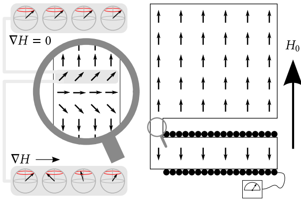
Figure 18. Helmholtz oscillations in a dilute mixture of liquid ^3\text{He} - ^4\text{He} explained by the formation and motion of a domain wall (left) in the narrow pipe connecting the top and the bottom container. This wall separates the spins which are aligned with the strong homogeneous magnetic field H_0 from the ones which are oriented against it due to an initial \pi -pulse created by a coil around the bottom container. The difference in size of the spin systems as well as their elasticity leads to an oscillatory motion of the wall detected by the coil as a current. The wall is strongly influenced by a gradient magnetic field \nabla H when aligned orthogonal to H_0 . Credit: Harald Losert.
