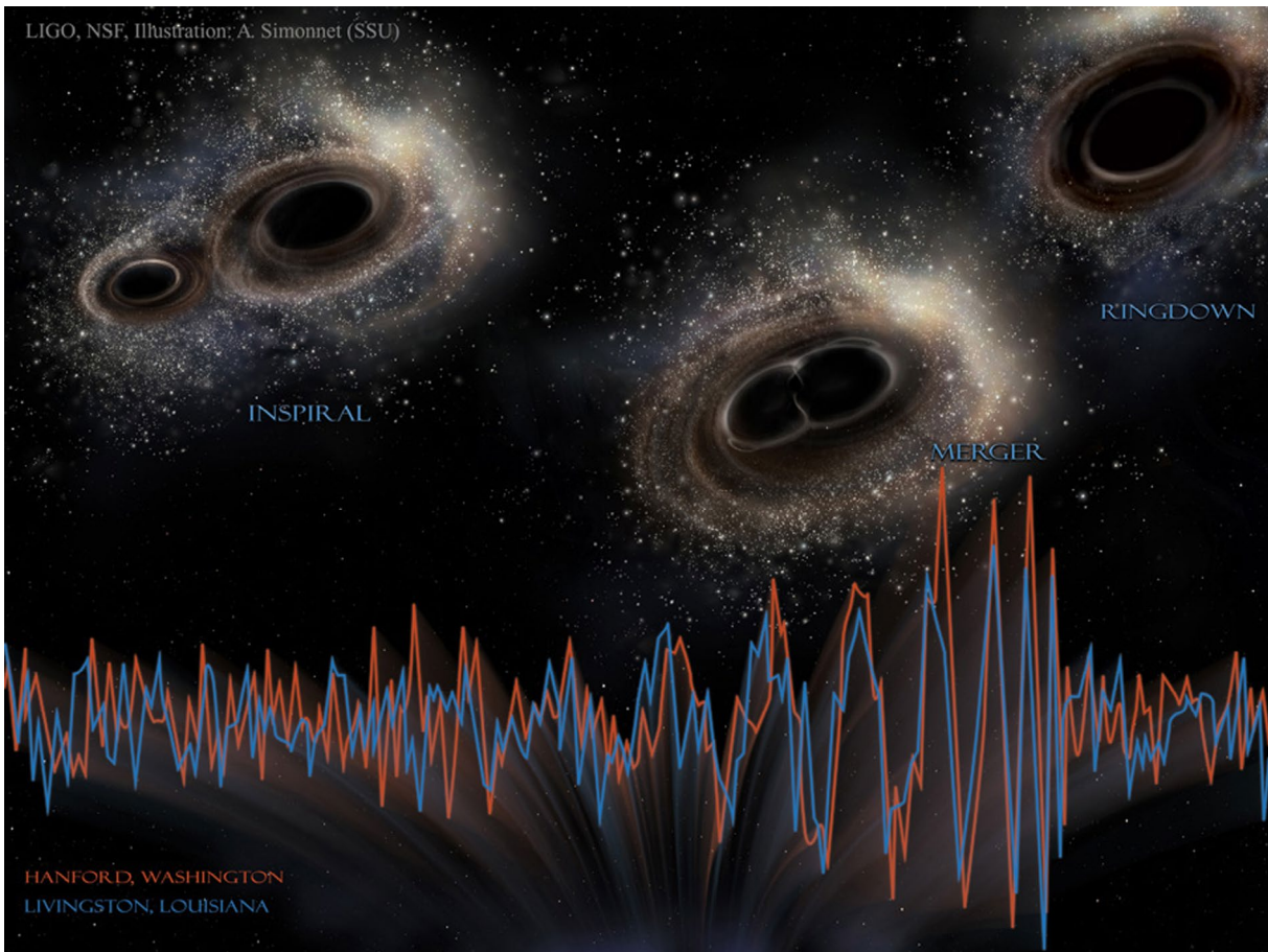
Figure 6. The LIGO collaboration has a spectacular double success: the first direct observation of gravitational waves – predicted by Einstein a century earlier – and the unexpected observation of the merger of two very massive black holes. As indicated in the figure, the waves were simultaneously detected at the two separate LIGO observatories in Hanford, Washington and Livingston, Louisiana, with amazingly consistent signals for the spiralling in and merger of the black holes, and the ringdown of the single remnant afterwards. This observation marks the beginning of gravitational wave astronomy. Credit: LIGO, NSF, Aurore Simonnet (Sonoma State U.).
