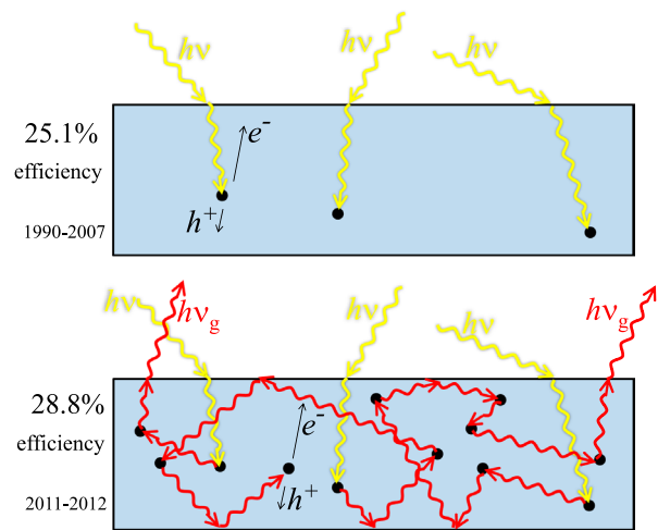
Figure 29. The physical picture of high efficiency solar cells, compared to conventional cells. In high efficiency solar cells, good luminescent extraction is a requirement for the highest open circuit voltages. One sun illumination is accompanied by up to 40 suns of trapped infrared luminescence, leading to the maximum external fluorescence efficiency. Credit: Eli Yablonovitch.
