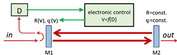
Figure 39. Maxwell’s demon for light: simplified schematics for the device envisioned and discussed in the text. Cavity mirror M1 is controlled electronically so as to minimize the total reflected power, while mirror M2 is fixed, ensuring stable monochromatic output. (Credit: Alexei V. Sokolov).
