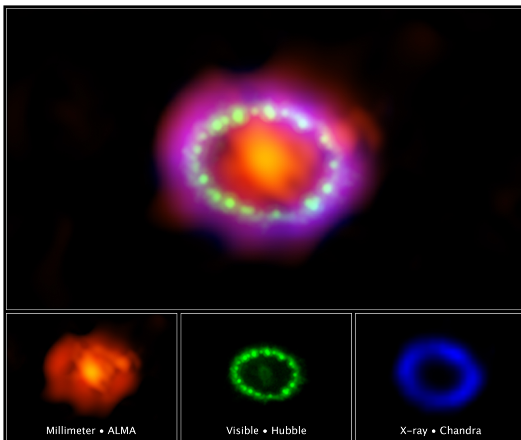
Figure 14. The remains of Supernova 1987A obtained by combining three observations from different telescopes/observatories (Credit: NASA, ESA and A. Angelich (NRAO/AUI/NSF)); the individual images are displayed in the lower part of the figure. On the left, in the millimetre range (Credit: ALMA; ESO/NAOJ/NRAO and R. Indebetouw (NRAO/AUI/NSF)), in the centre, the Hubble Telescope measurements in the visible range (Credit: NASA, ESA and R. Kirshner (Harvard-Smithsonian Centre for Astrophysics and Gordon and Betty Moore Foundation)) and on the right, an image in the X-ray spectrum from Chandra. Credit: NASA/CXC/Penn State/K. Frank et al. https://www.nasa.gov/sites/default/files/thumbnails/image/stsci-h-p1708b-f-3000x2500.jpg
