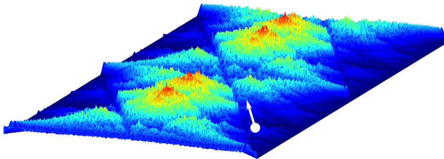
Figure 17. Fractal Smith–Purcell radiation emitted by an electron passing by a rough metal surface provided for example by a fractal quantum carpet. Credit: Harald Losert.
