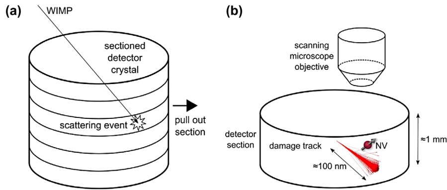
Figure 26. (a) Sectioned detector: Event identified by conventional methods. The section of interest is studied separately in (b). (b) Superresolution techniques applied to sense the localized crystal damage optically. Credit: Surjeet Rajendran.
