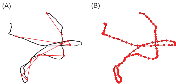
Figure 1 (online color at: www.ann-phys.org ) A 2D trajectory of a Brownian particle. The black curve is assumed to be a true trajectory of the particle. Red dots are measured positions, and red curves are measured trajectories. The sampling rate of (B) is 10 times of that of (A).
