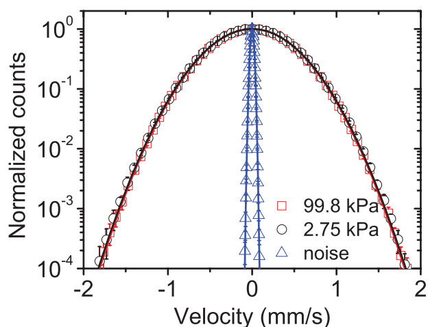
Figure 5 (online color at: www.ann-phys.org ) The distribution of the measured instantaneous velocities of a 3 \mu\text{m} silica bead. The statistics at each pressure are calculated from 4 million instantaneous velocities. The solid lines are Maxwell-Boltzmann distributions. Figure adapted from Ref. [21].
