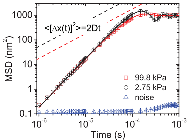
Figure 4 (online color at: www.ann-phys.org ) The mean square displacements of a 3 \mu\text{m} silica bead trapped in air at 99.8 kPa (red square) and 2.75 kPa (black circle). The solid lines are the theoretical predictions of Eq. (11). The prediction of Einstein's theory of free Brownian motion in the diffusive regime is shown in dashed lines for comparison. Figure adapted from Ref. [21].
