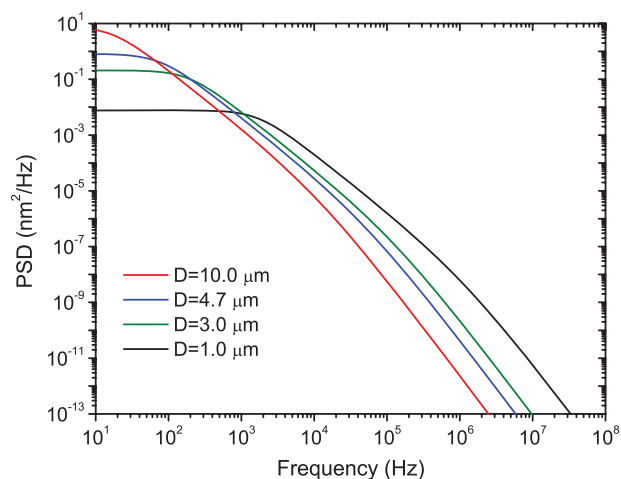
Figure 9 (online color at: www.ann-phys.org ) Calculated power spectra of an optically trapped silica microsphere in water at 20 °C. Parameters are the same as those in Table 1.
