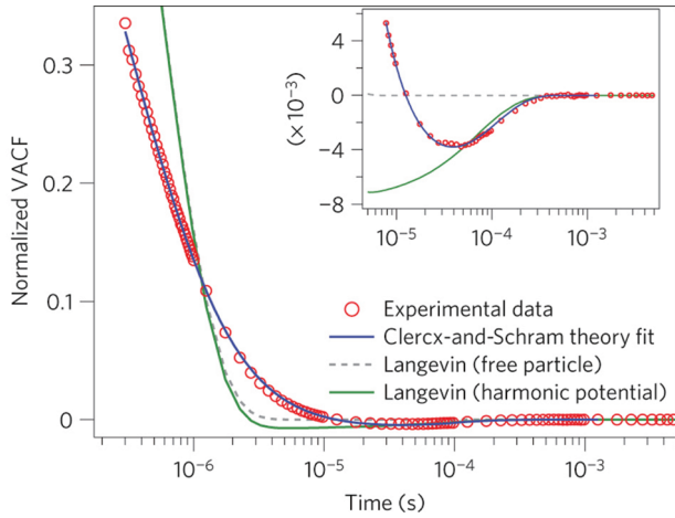
Figure 13 (online color at: www.ann-phys.org ) Normalized experimental VACF for a 2 \mu\text{m} diameter resin sphere in an optical trap (Figure adapted from Ref. [24]). The blue line shows the fitting of the Clercx-and-Schram theory (Eq. (26)) to the whole experimental VACF. The grey (dashed) and green lines show the expectations of VACF for the same particle if the inertia of the liquid is ignored, in the absence (grey) and presence (green) of the harmonic trap.
