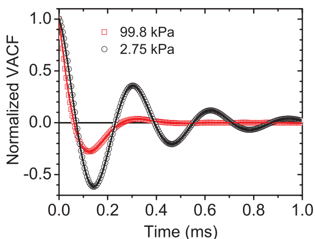
Figure 6 (online color at: www.ann-phys.org ) The normalized velocity autocorrelation functions of the 3 \mu\text{m} bead at 99.8 kPa (red square) and at 2.75 kPa (black circle) from the measurements. The solid lines are fittings with Eq. (14). Figure adapted from Ref. [21].
