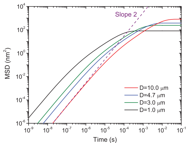
Figure 8 (online color at: www.ann-phys.org ) Calculated mean square displacement of an optically trapped silica microsphere in water at 20 °C. Parameters are the same as those in Table 1.
