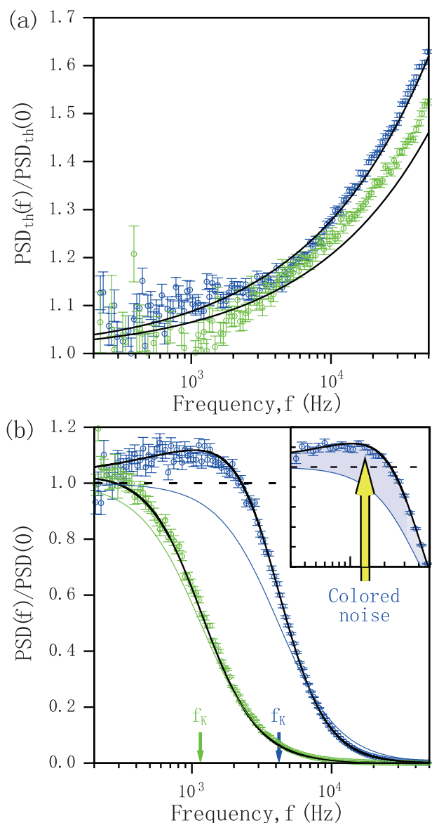
Figure 11 (online color at: www.ann-phys.org ) The color of thermal force (Figure adapted from Ref. [25]). (a), The normalized power spectral density (PSD) of thermal force of an optically trapped melamine resin sphere ( R = 1.45 \mu\text{m} ) in water (green circles) or acetone (blue circles). The black lines are predictions of the hydrodynamic theory. (b), The normalized power spectral density of position.
