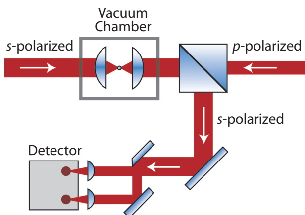
Figure 2 (online color at: www.ann-phys.org ) This simplified schematic shows our counter-propagating dual-beam optical tweezers, and a novel detection system (Figure adapted from Ref. [21]). The s -polarized beam is reflected by a polarizing beam splitter cube after it passes through a trapped bead inside a vacuum chamber. Then, for detection, it is split by a mirror with a sharp edge. The p -polarized beam passes through the cube.
