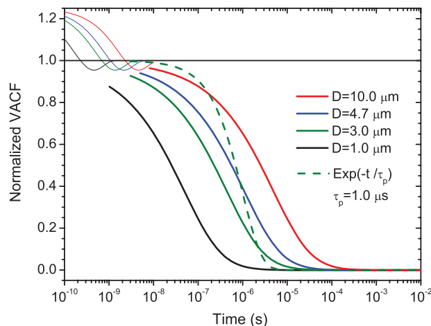
Figure 10 (online color at: www.ann-phys.org ) Calculated normalized velocity autocorrelation function of an optically trapped silica microsphere in water at 20 °C. Parameters are the same as those in Table 1. The thin solid lines ( t < 10^{-8} s) are calculated from Eq. (28), and the thick solid lines are calculated from Eq. (26). The dashed lines are exponential decays with \tau_p = 1.0 \mu\text{s} , corresponding to a 3.0 \mu\text{m} microsphere.
