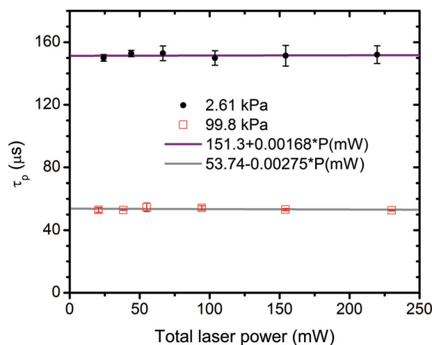
Figure 7 (online color at: www.ann-phys.org ) Measured momentum relaxation times ( \tau_p ) of a microsphere trapped at 2.61 kPa and 99.8 kPa as a function of the total power of the two trapping beams.
