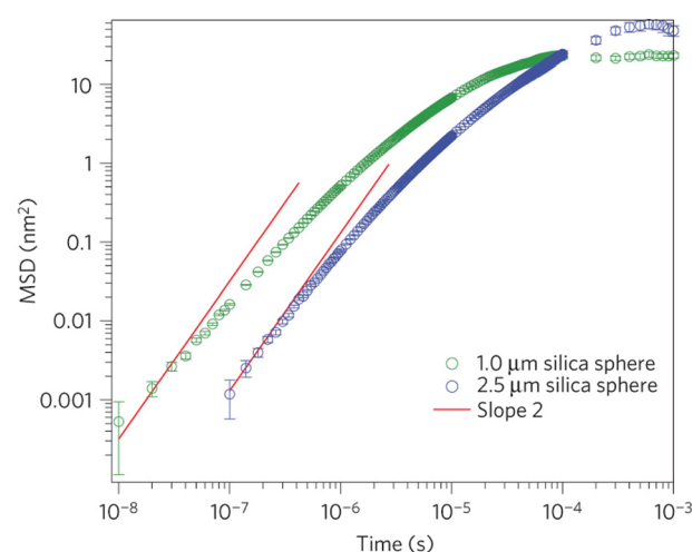
Figure 12 (online color at: www.ann-phys.org ) Measured mean square displacement of silica spheres with diameters of 1 \mu\text{m} and 2.5 \mu\text{m} (Figure adapted from Ref. [24]). The red lines with slope 2 show the expected behavior of ballistic Brownian motion.
