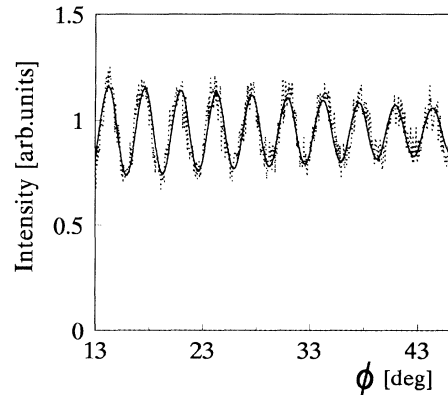
FIG. 3. Shown are the interference fringes for d = 3.35 \ \mu\text{m} together with a fit to the data. For these data, the temperature of the ions was determined to be 1.5 times higher than the temperature at the Doppler-cooling limit.
